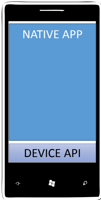
Native App
