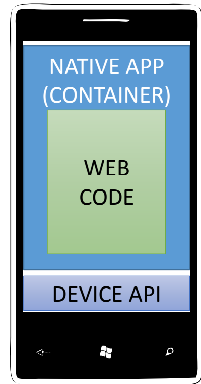
Hybrid-Application
